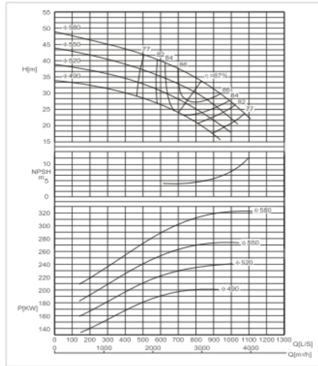
SBS500-640 F Performance Curve n=960r/min
