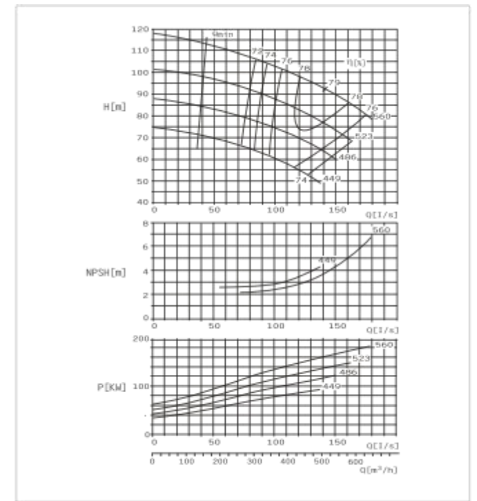
SBS150-605 F Performance Curve n=1450r/min
