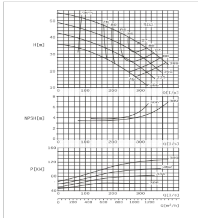
SBS250-370 F Performance Curve n=1450r/min
