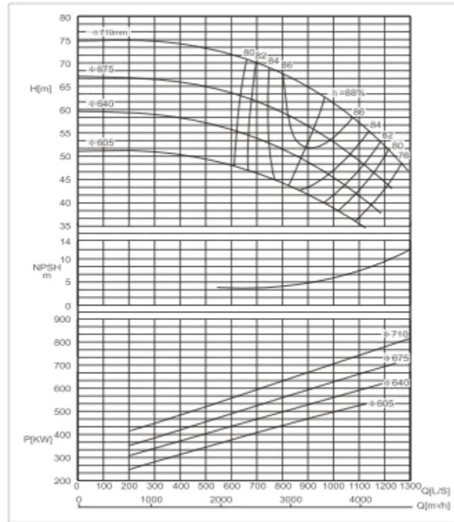
SBS500-790 F Performance Curve n=960r/min
