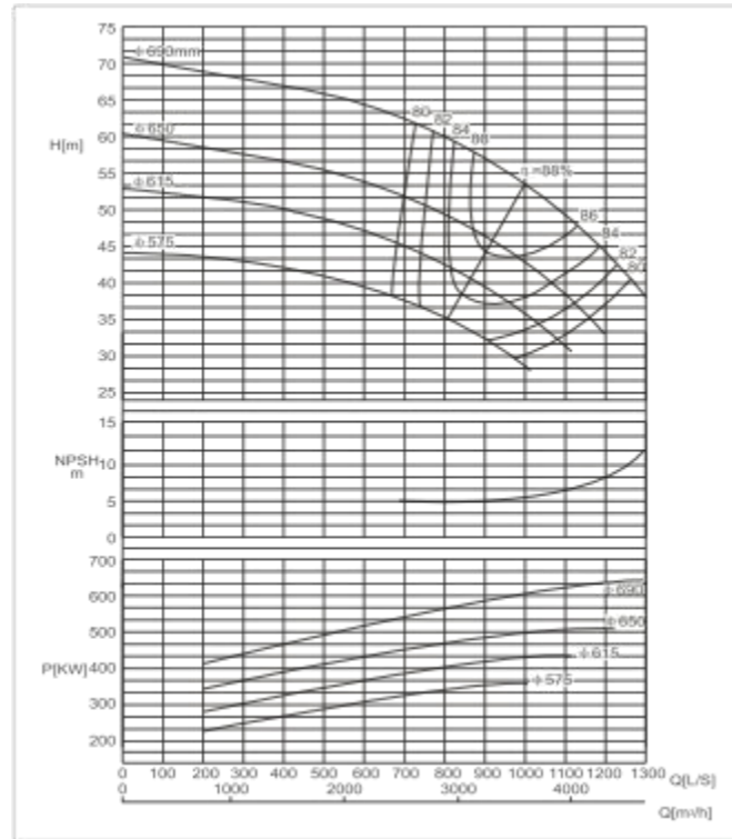
SBS600-710 F Performance Curve n=960r/min
