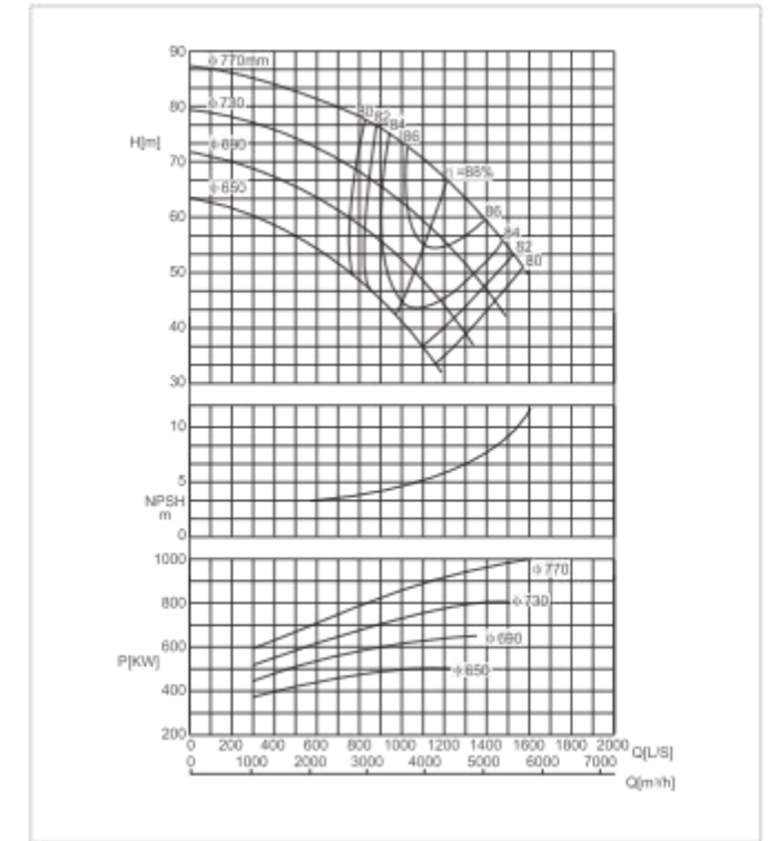
SBS600-830 F Performance Curve n=960r/min
