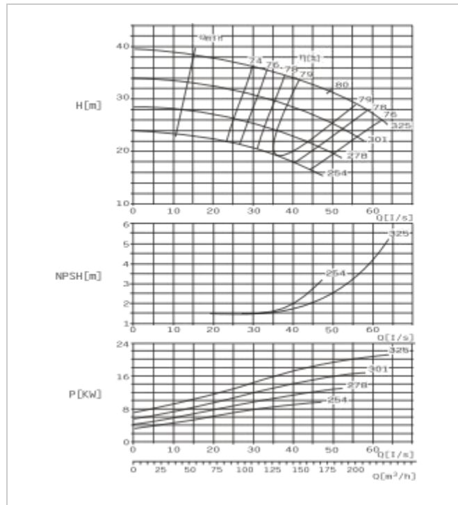
SBS100-310 E Performance Curve n=1450r/min
