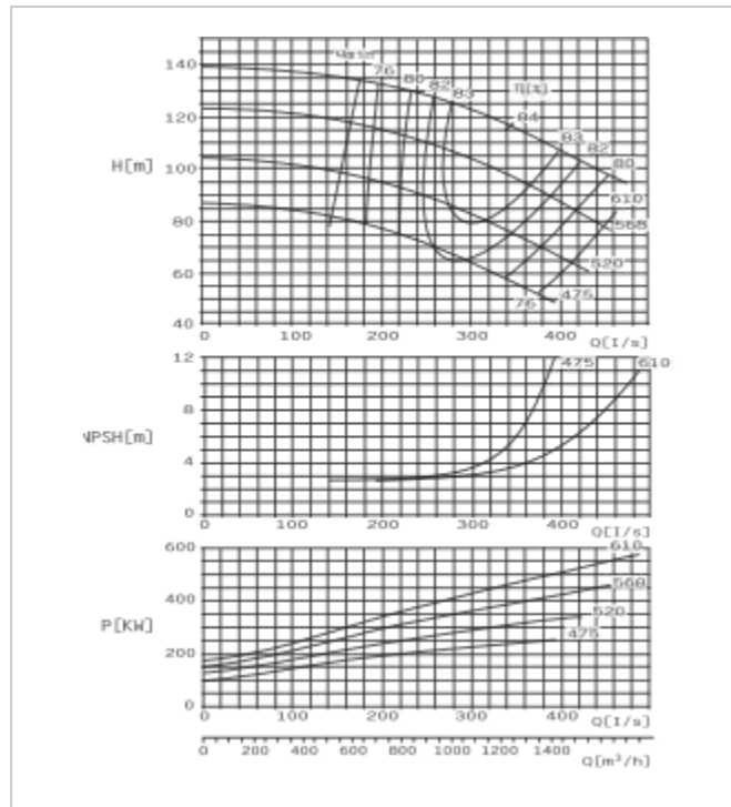
SBS250-600 E Performance Curve n=1450r/min
