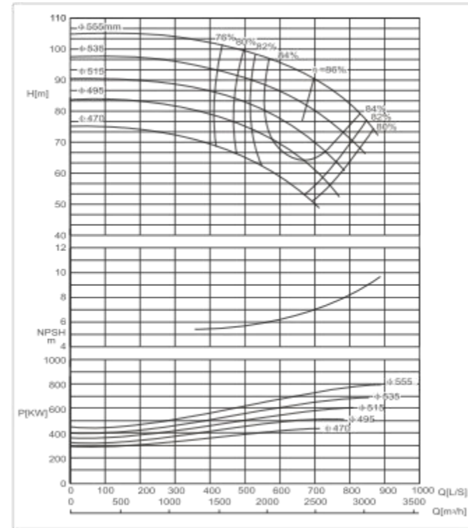
SBS400-620 F Performance Curve n=1450r/min
