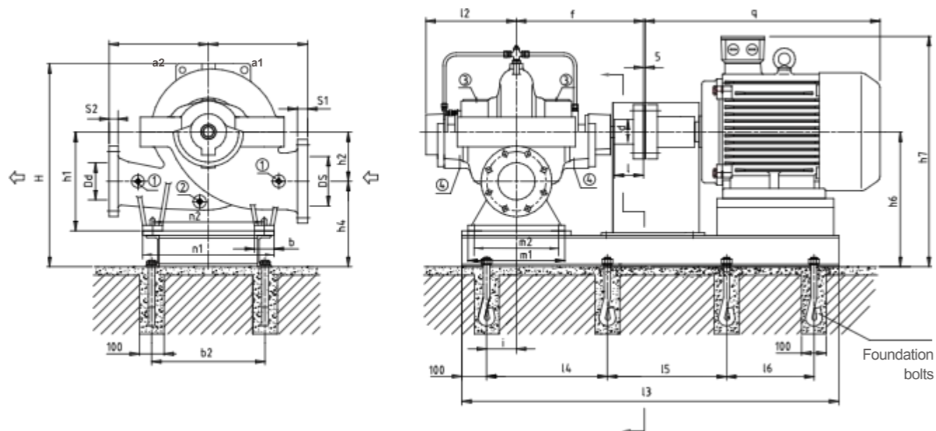
Suction flange
