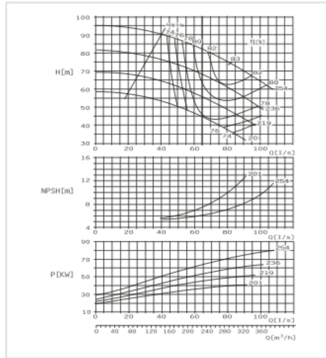
SBS100-250 EG Performance Curve n=2900r/min
