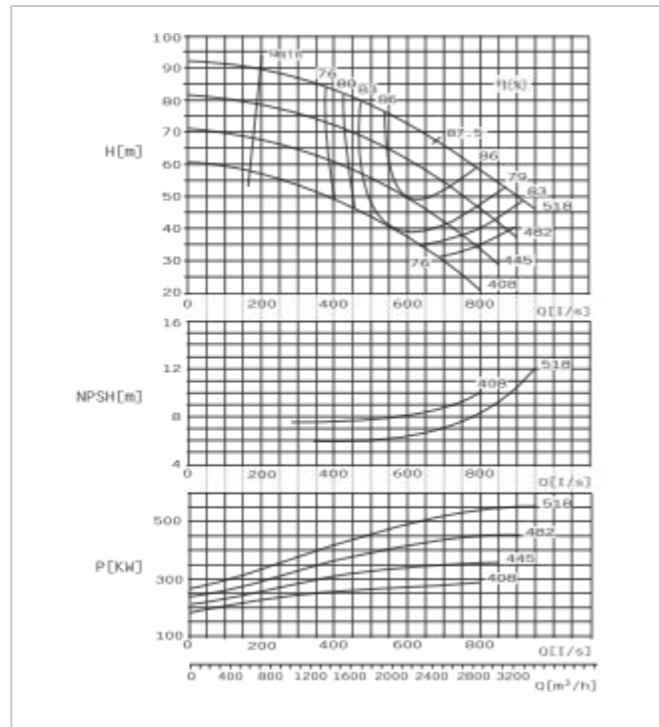
SBS350-510 F Performance Curve n=1450r/min
