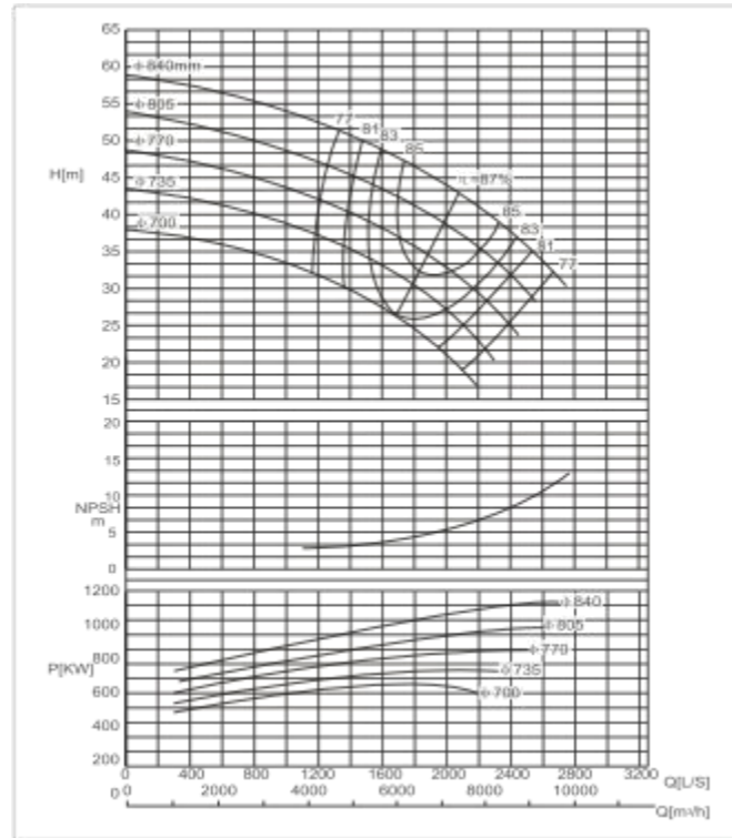
SBS800-840 F Performance Curve n=725r/min
