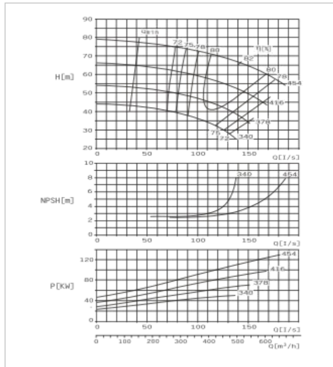
SBS150-460 E Performance Curve n=1450r/min
