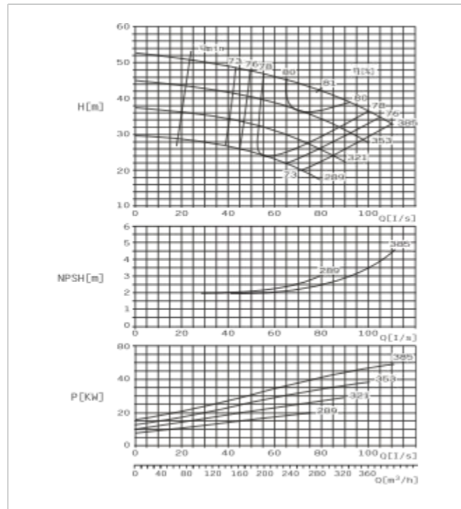
SBS125-365 F Performance Curve n=1450r/min
