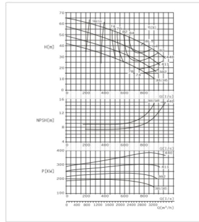
SBS350-430 E Performance Curve n=1450r/min
