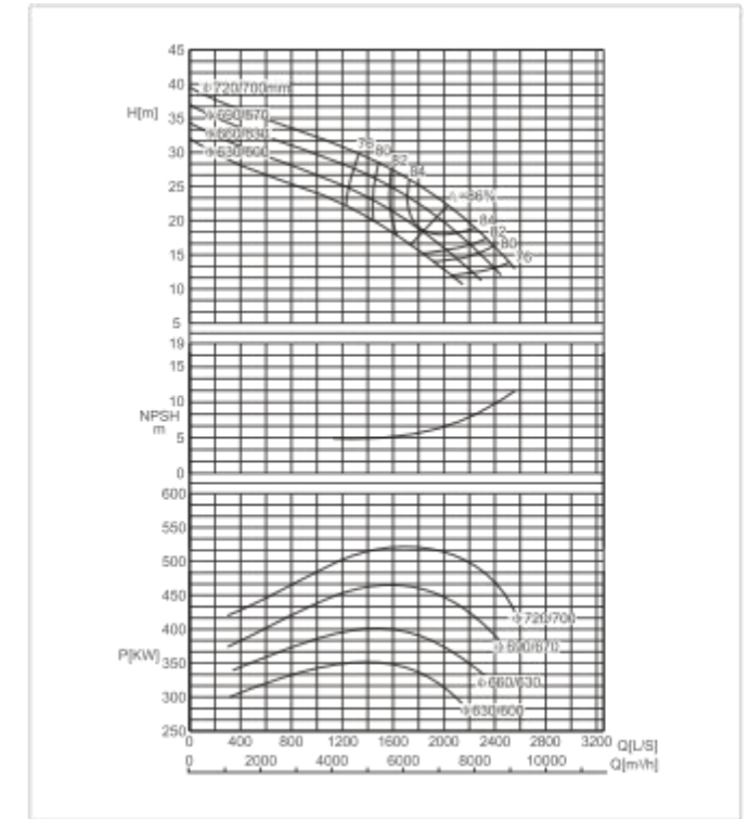
SBS800-740 F Performance Curve n=725r/min
