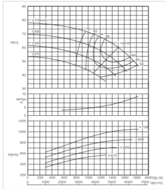
SBS700-820 F Performance Curve n=960r/min
