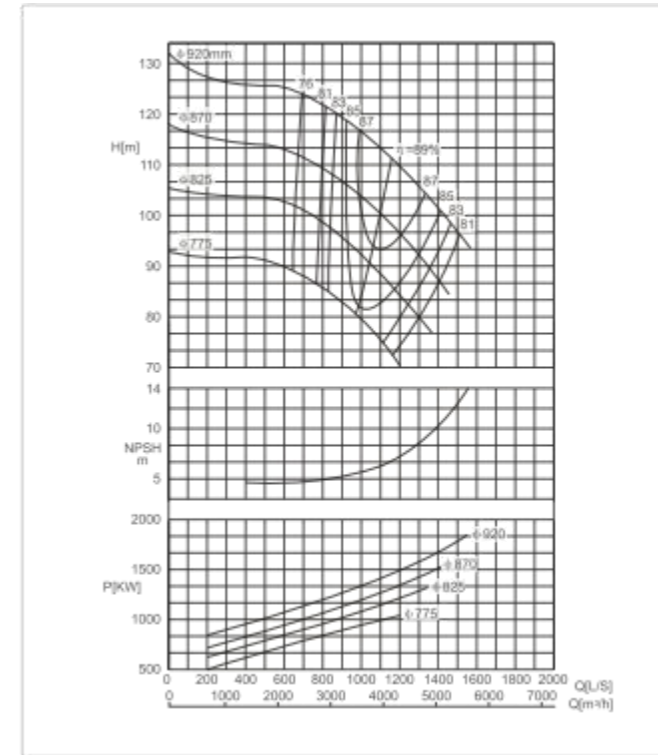
SBS500-890 E Performance Curve n=960r/min
