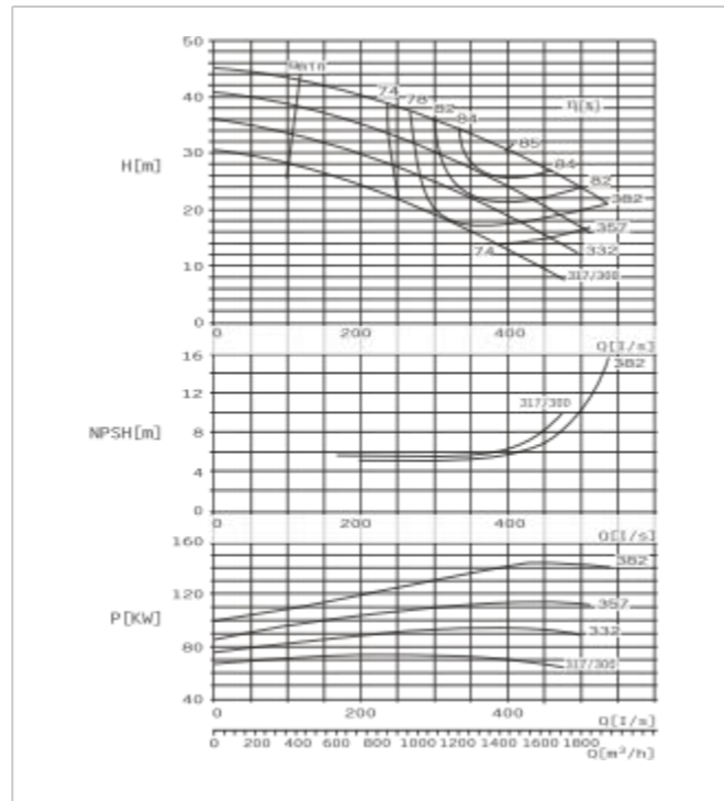
SBS350-360 F Performance Curve n=1450r/min
