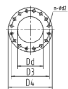
Suction flange
