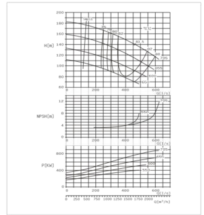
SBS300-700 F Performance Curve n=1450r/min
