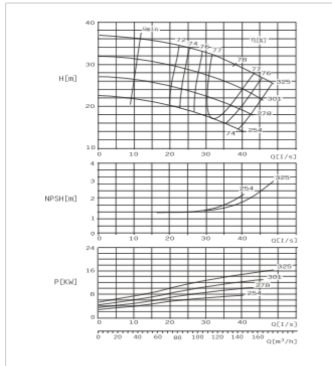
SBS100-310 F Performance Curve n=1450r/min
