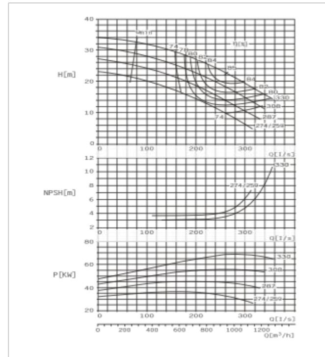
SBS300-300 F Performance Curve n=1450r/min
