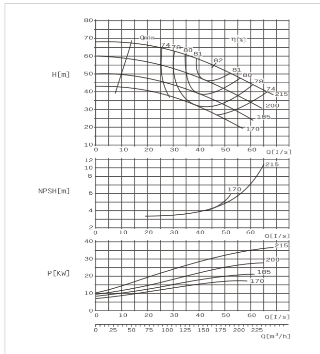
SBS80-210 EG Performance Curve n=2900r/min
