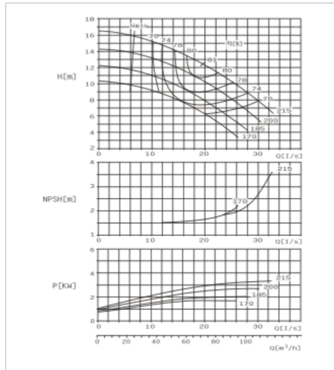
SBS80-210 F Performance Curve n=1450r/min
