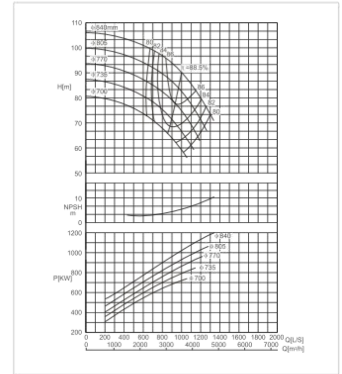
SBS500-890 F Performance Curve n=960r/min
