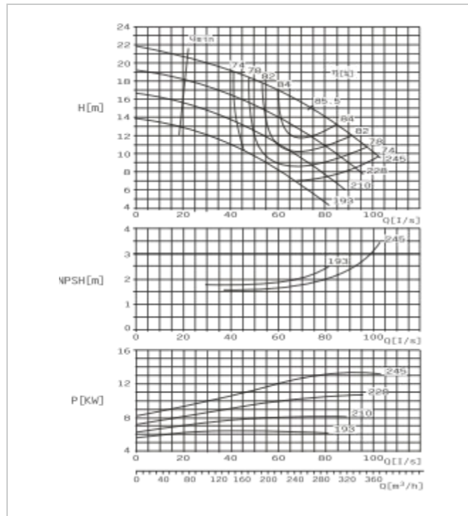
SBS125-230 E Performance Curve n=1450r/min
