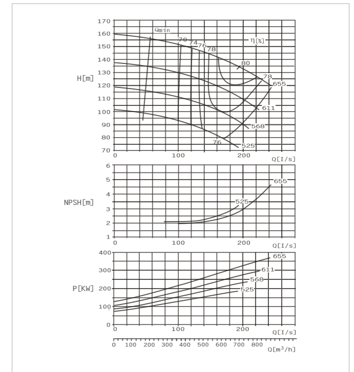
SBS200-670 F Performance Curve n=1450r/min
