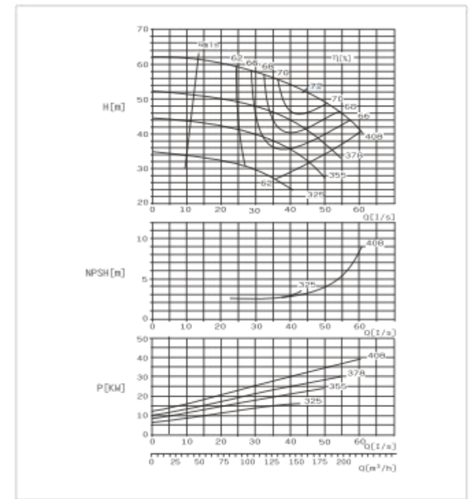
SBS100-375 F Performance Curve n=1450r/min
