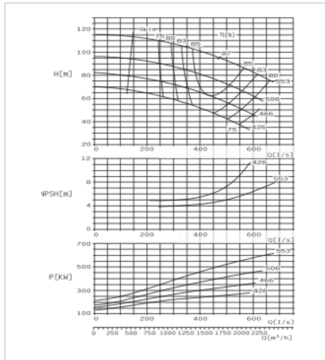
SBS300-560 E Performance Curve n=1450r/min
