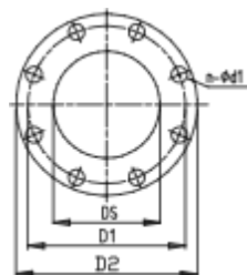
Suction flange
