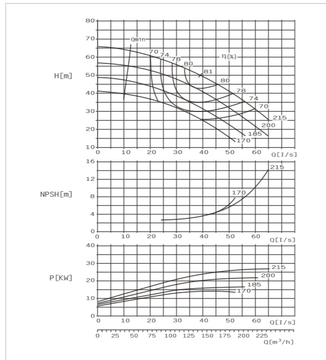
SBS80-210 FG Performance Curve n=2900r/min
