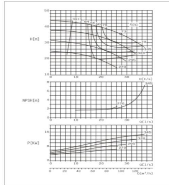
SBS80-370 F Performance Curve n=1450r/min
