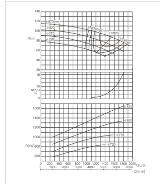
SBS600-830 E Performance Curve n=960r/min
