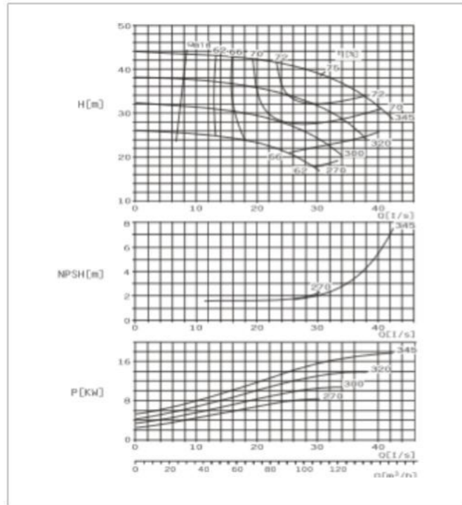
SBS80-370 E Performance Curve n=1450r/min
