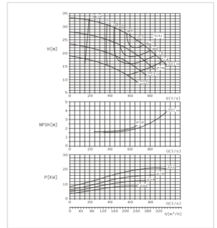
SBS125-290 F Performance Curve n=1450r/min
