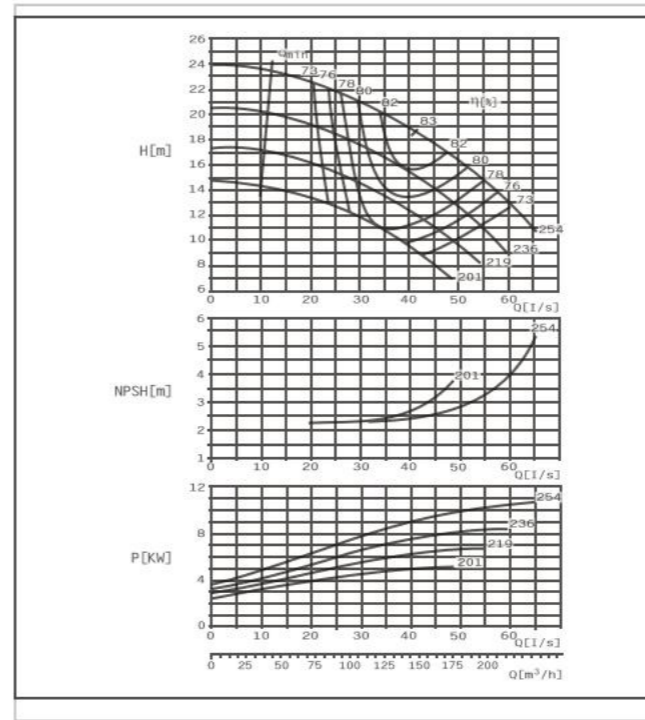
SBS100-250 E Performance Curve n=1450r/min
