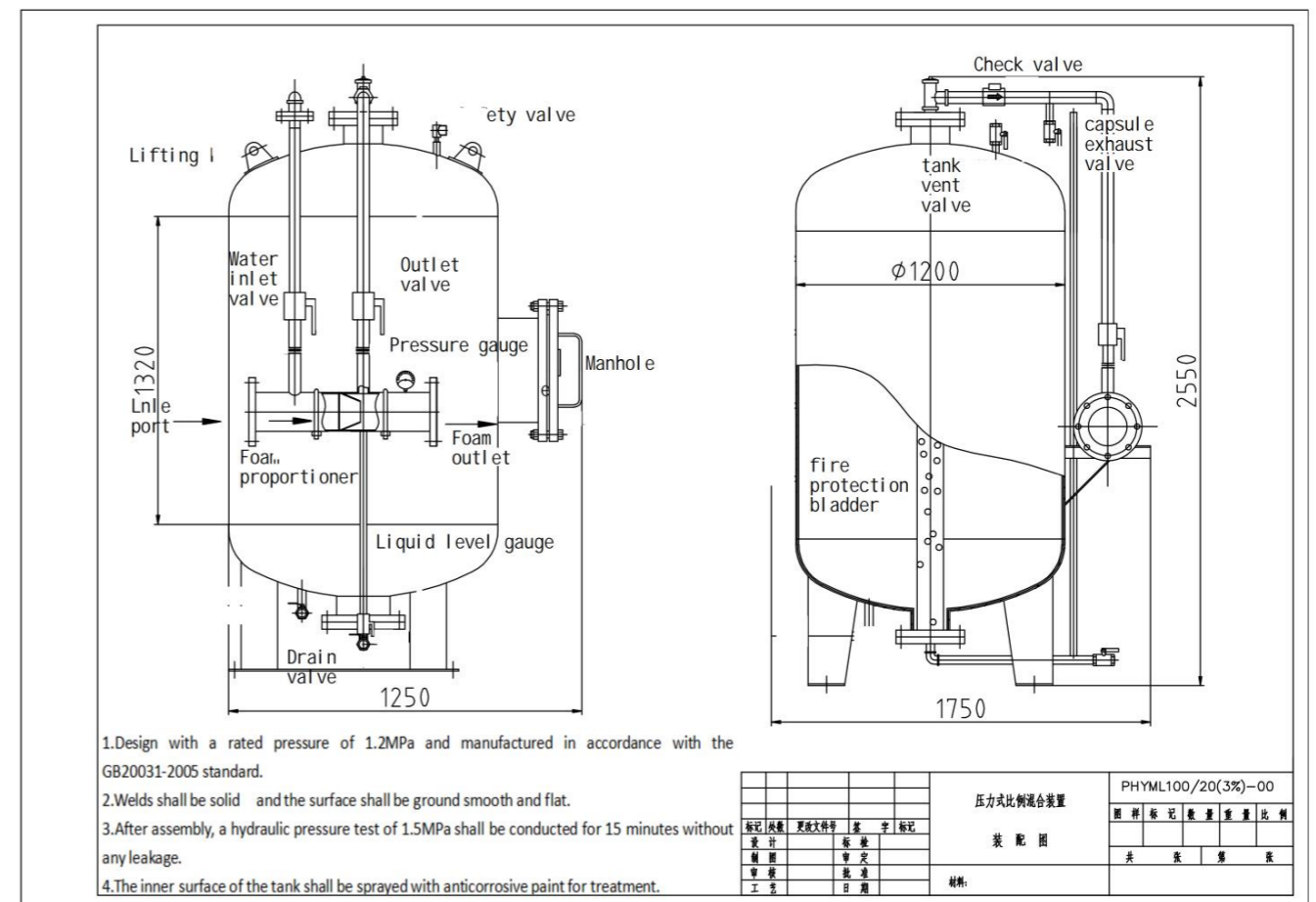
Vertical Foam Tank
