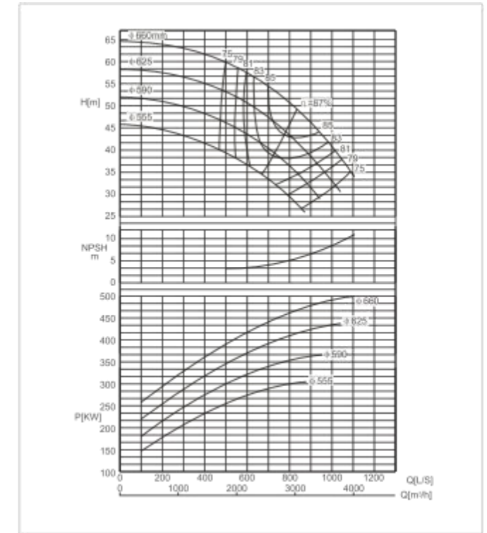
SBS500-700 F Performance Curve n=960r/min
