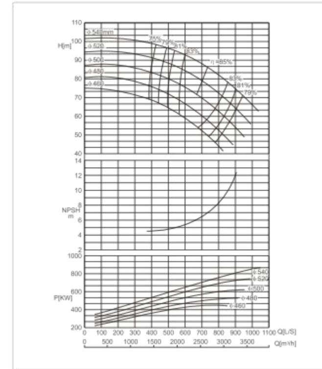
SBS400-540 E Performance Curve n=1450r/min
