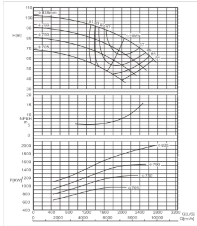
SBS700-820 E Performance Curve n=960r/min
