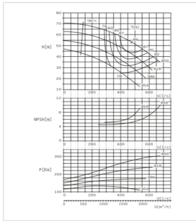
SBS300-435 E Performance Curve n=1450r/min
