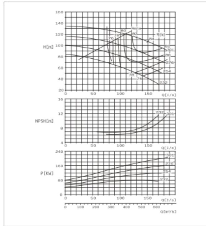
SBS125-290 EG Performance Curve n=2900r/min
