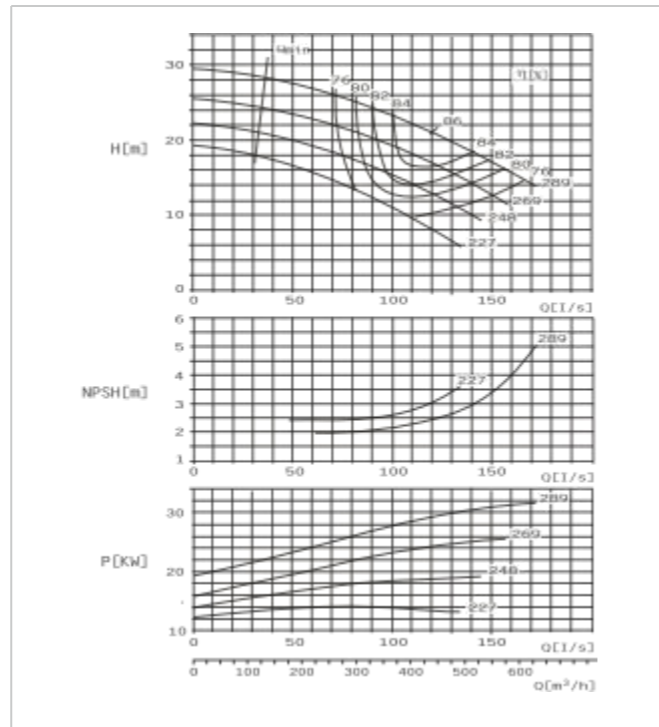
SBS150-290 F Performance Curve n=1450r/min
