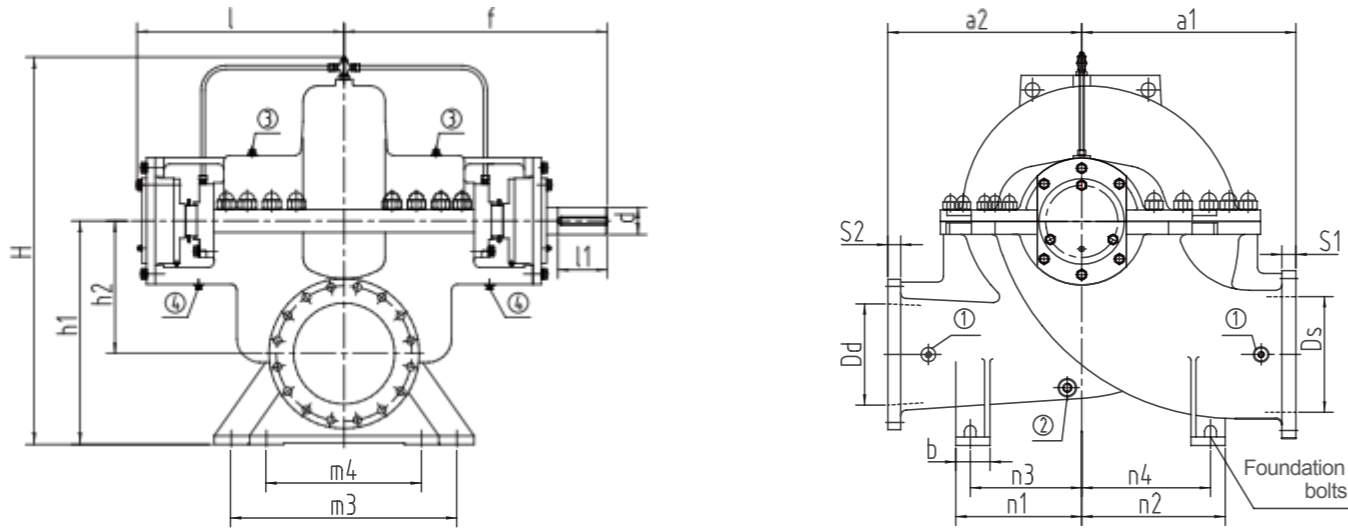
Suction flange
