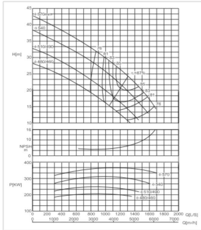
SBS600-540 E Performance Curve n=960r/min
