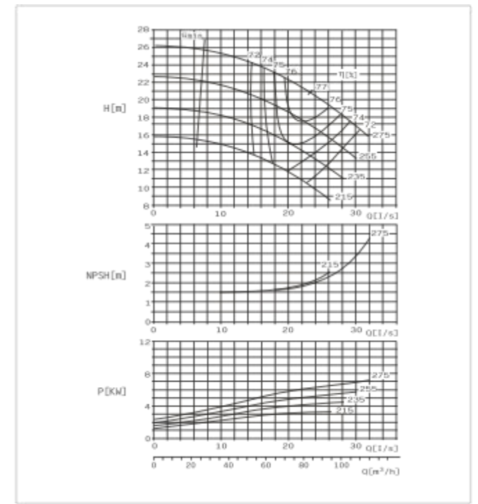
SBS80-270 F Performance Curve =1450r/min
