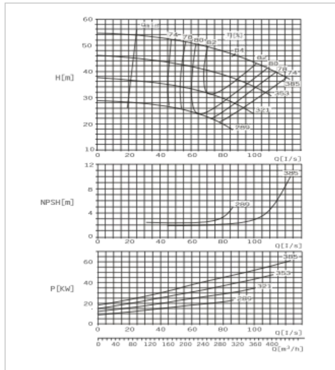
SBS125-365 E Performance Curve n=1450r/min
