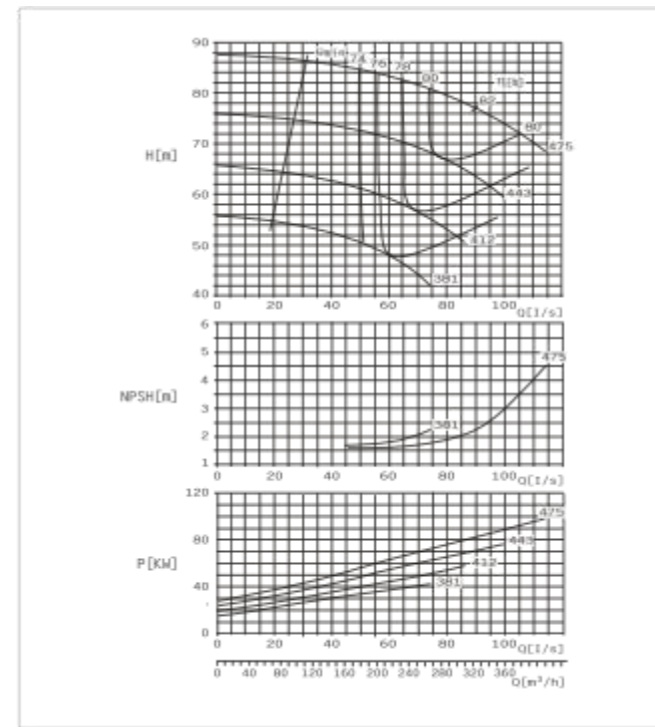
SBS125-500 E Performance Curve n=1450r/min
