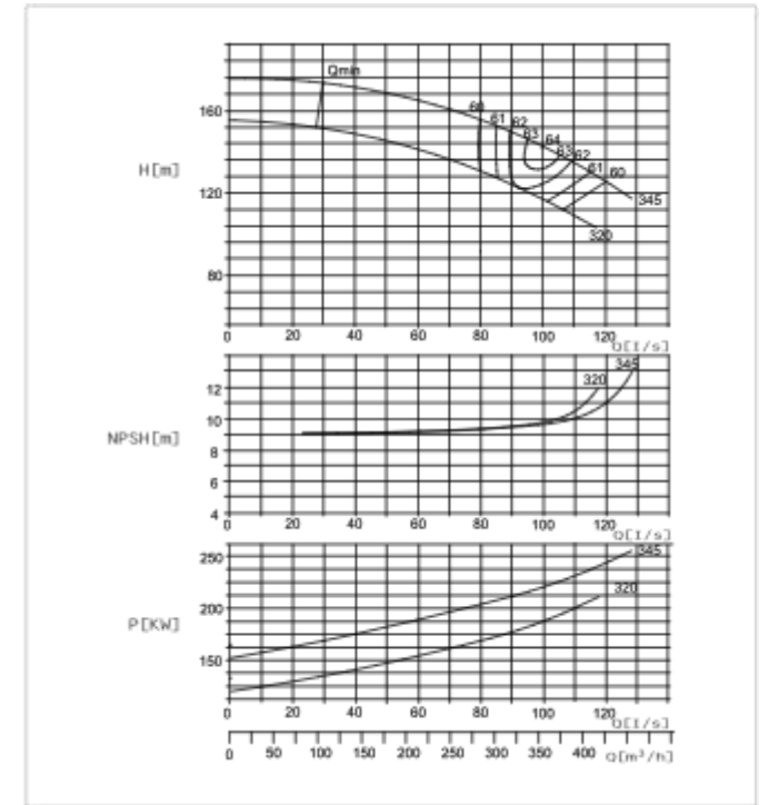
SBS100-345 EG Performance Curve n=2900r/min
