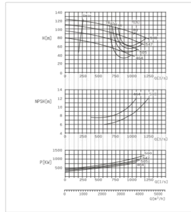
SBS350-590 E Performance Curve n=1450r/min
