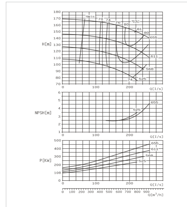
SBS200-670 E Performance Curve n=1450r/min
