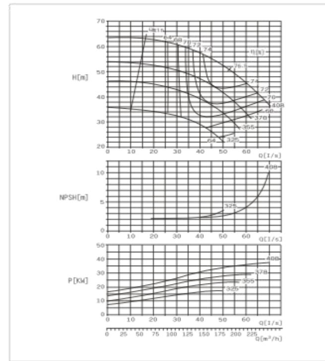
SBS100-375 E Performance Curve n=1450r/min
