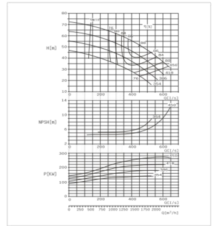
SBS300-435 F Performance Curve n=1450r/min
