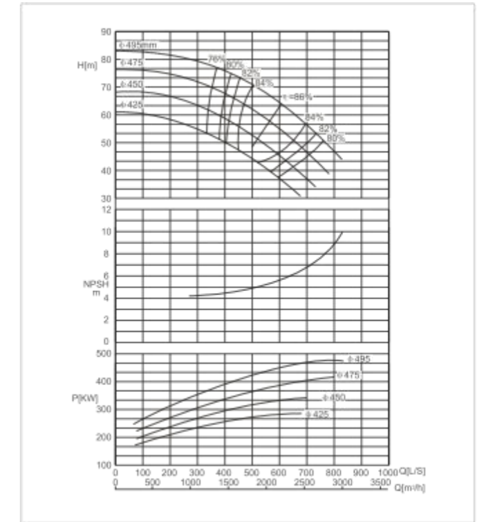
SBS400-540 F Performance Curve n=1450r/min
