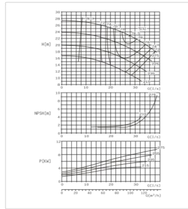
SBS80-270 E Performance Curve n=1450r/min
