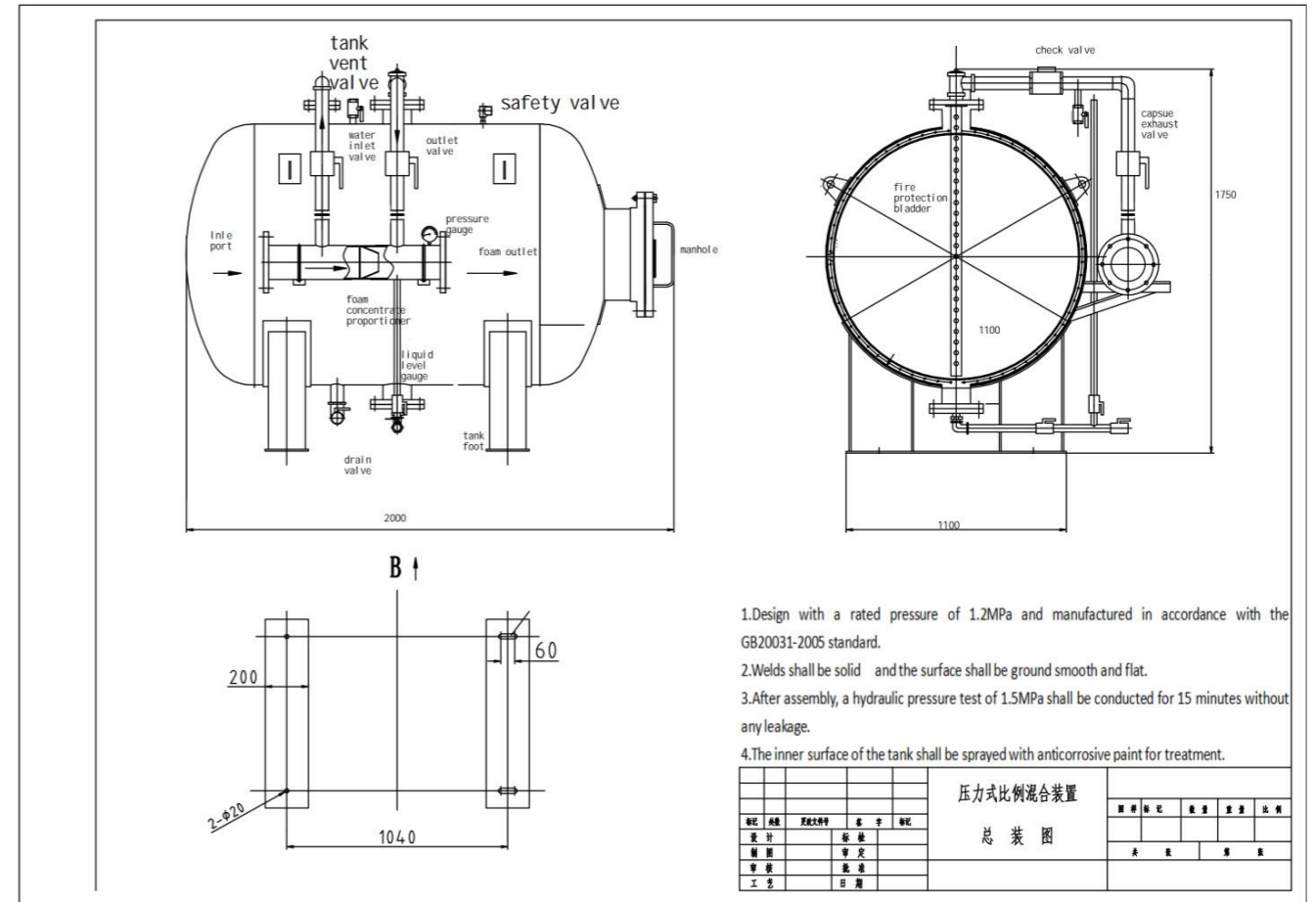
Horizontal Foam Tank
