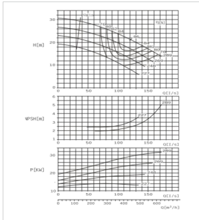
SBS150-290 E Performance Curve n=1450r/min
