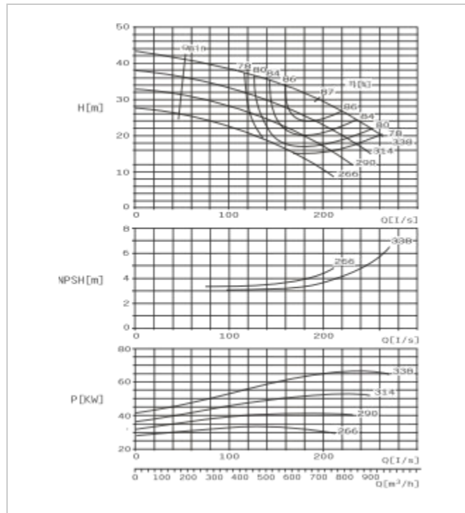
SBS200-320 E Performance Curve n=1450r/min
