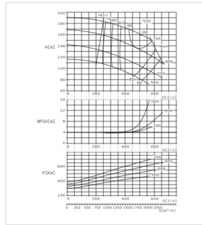
SBS300-700 E Performance Curve n=1450r/min
