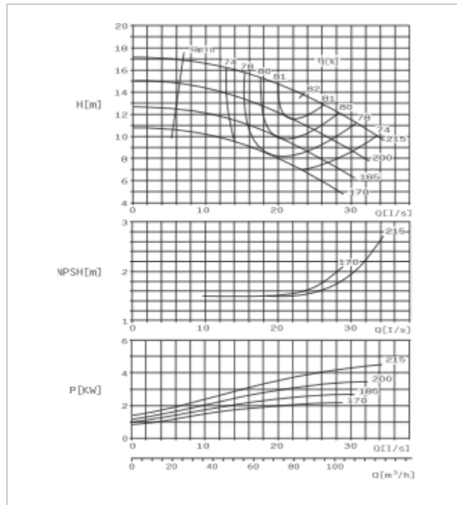
SBS80-210 E Performance Curve n=1450r/min
