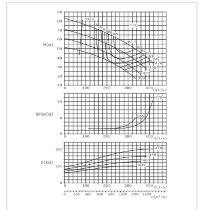
SBS250-480 F Performance Curve n=1450r/min
