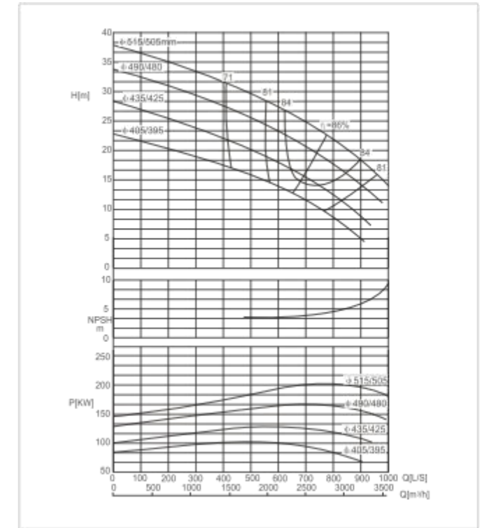
SBS500-510 F Performance Curve n=960r/min
