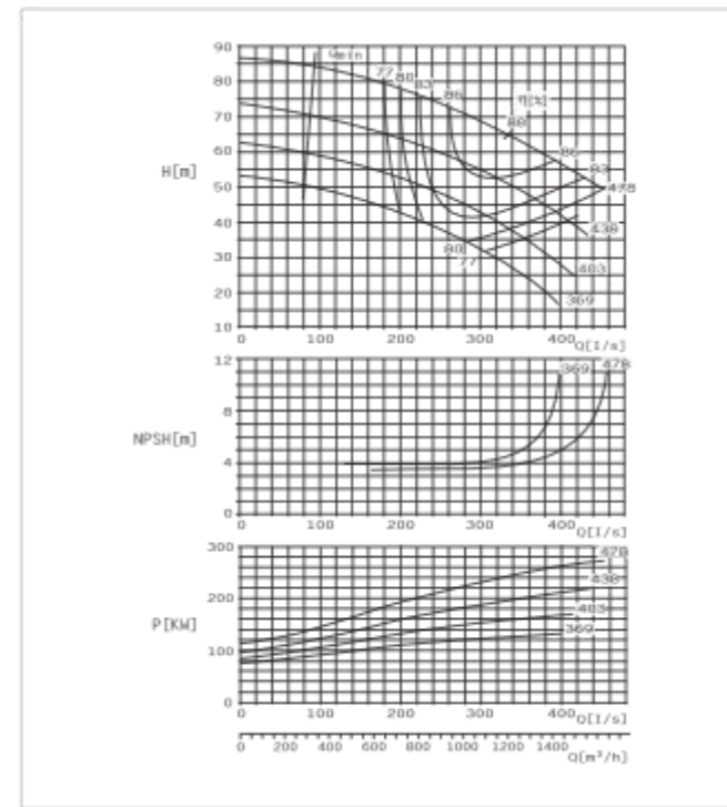
SBS250-480 E Performance Curve n=1450r/min
