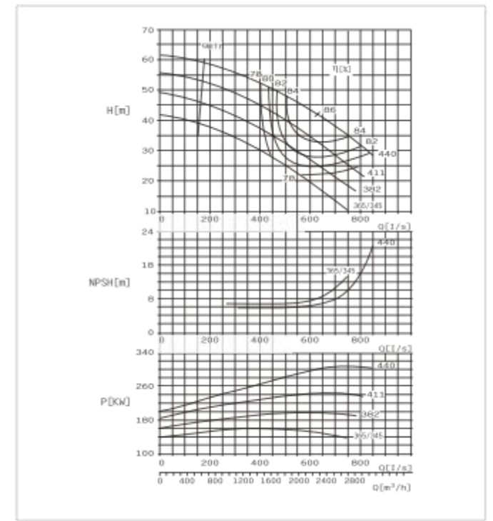
SBS350-430 F Performance Curve n=1450r/min
