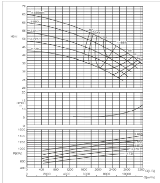
SBS800-840 E Performance Curve n=725r/min
