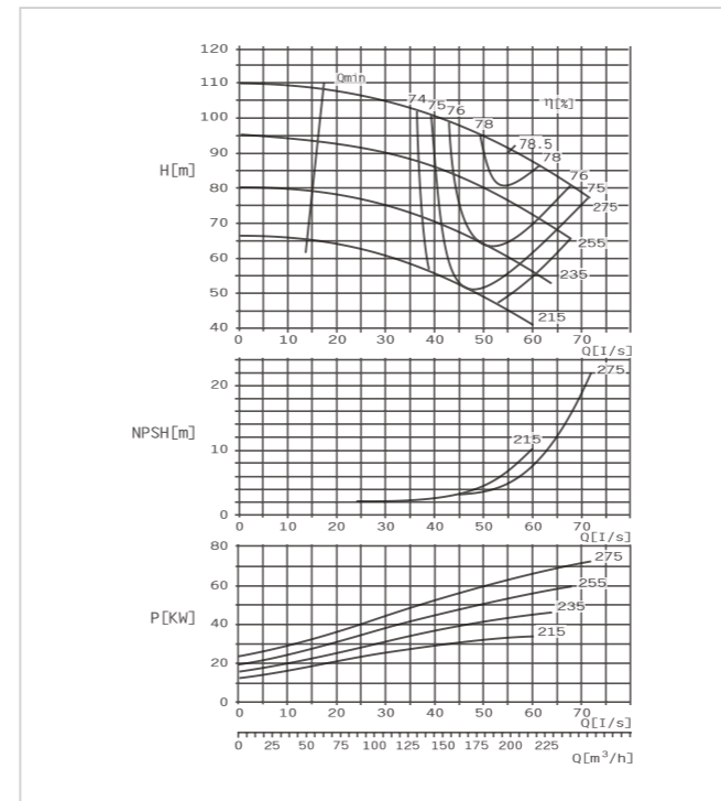
SBS80-270 EG Performance Curve n=2900r/min
