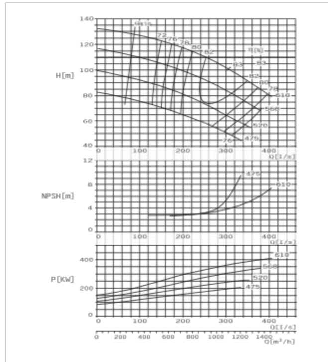
SBS250-600 F Performance Curve n=1450r/min
