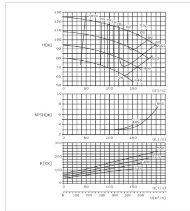
SBS150-605 E Performance Curve n=1450r/min
