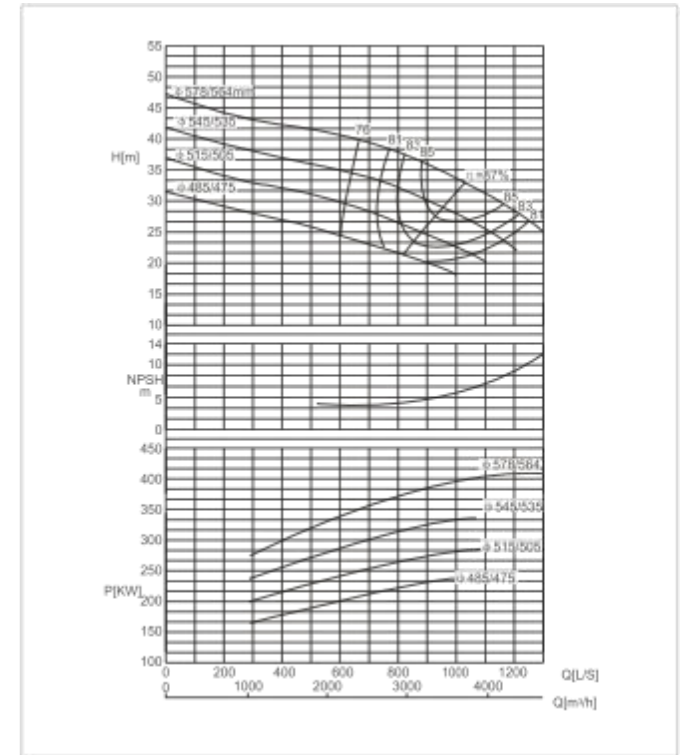
SBS600-620 F Performance Curve n=960r/min
