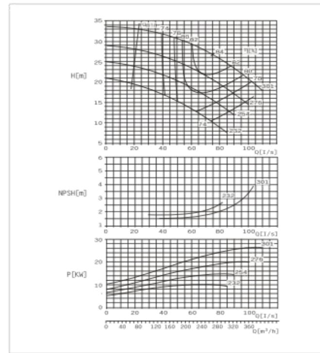
SBS125-290 E Performance Curve n=1450r/min
