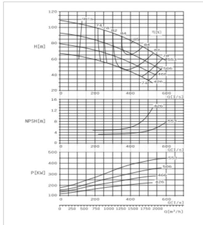
SBS300-560 F Performance Curve n=1450r/min
