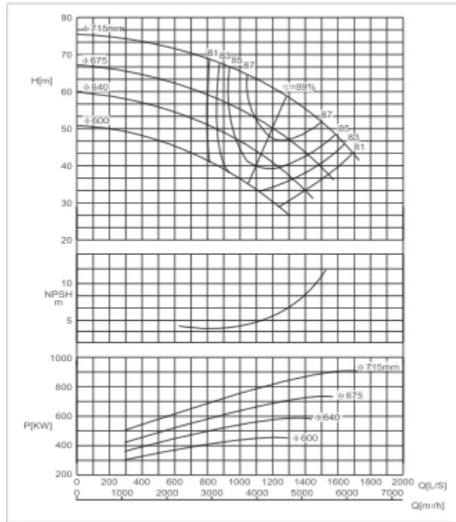
SBS600-710 E Performance Curve n=960r/min
