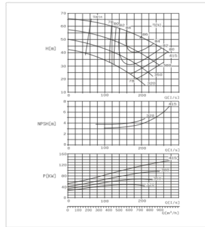
SBS200-420 E Performance Curve n=1450r/min
