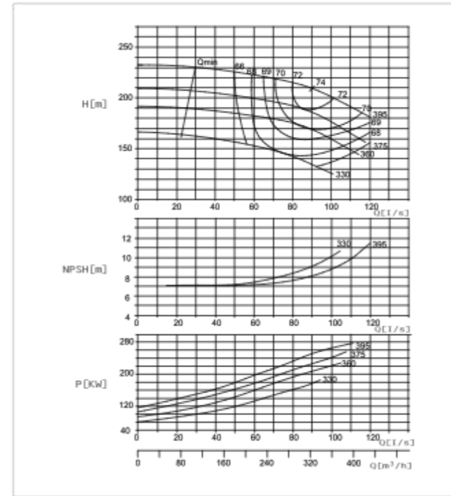
SBS125-400 EG Performance Curve n=2900r/min
