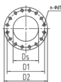
Suction flange
