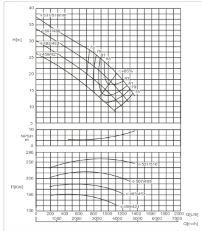
SBS600-540 F Performance Curve n=960r/min
