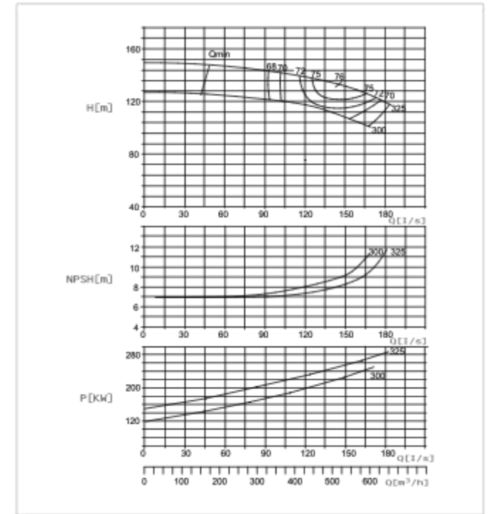
SBS150-330 EG Performance Curve n=2900r/min
