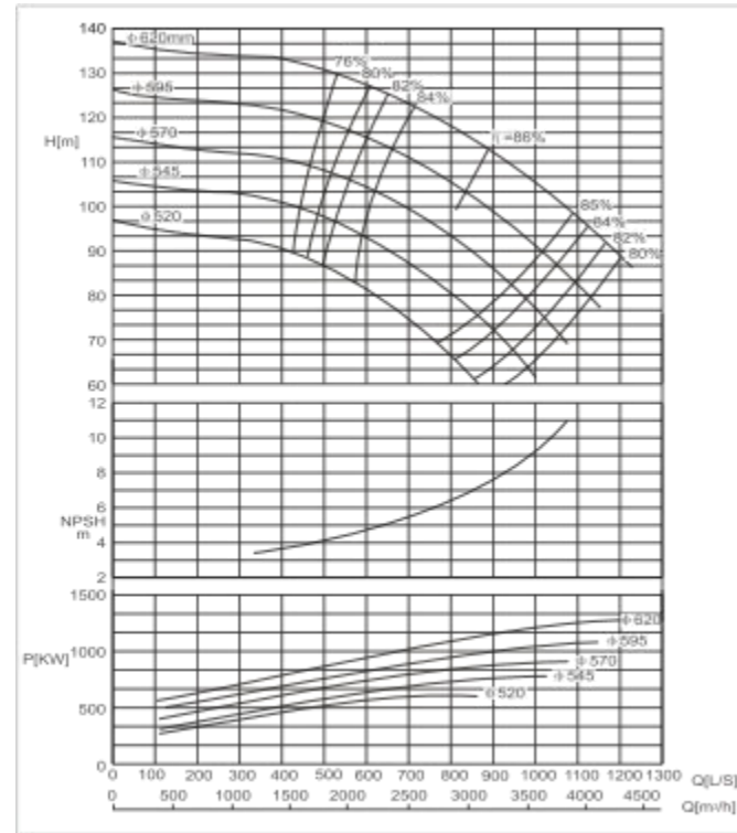
SBS400-620 E Performance Curve n=1450r/min
