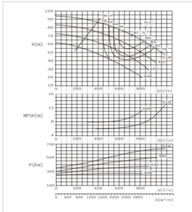
SBS350-510 E Performance Curve n=1450r/min
