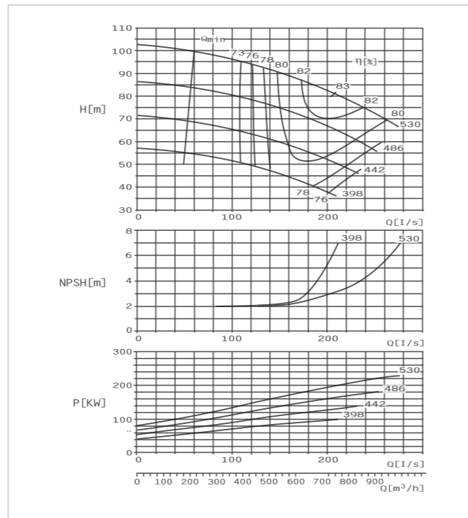
SBS200-520 F Performance Curve n=1450r/min
