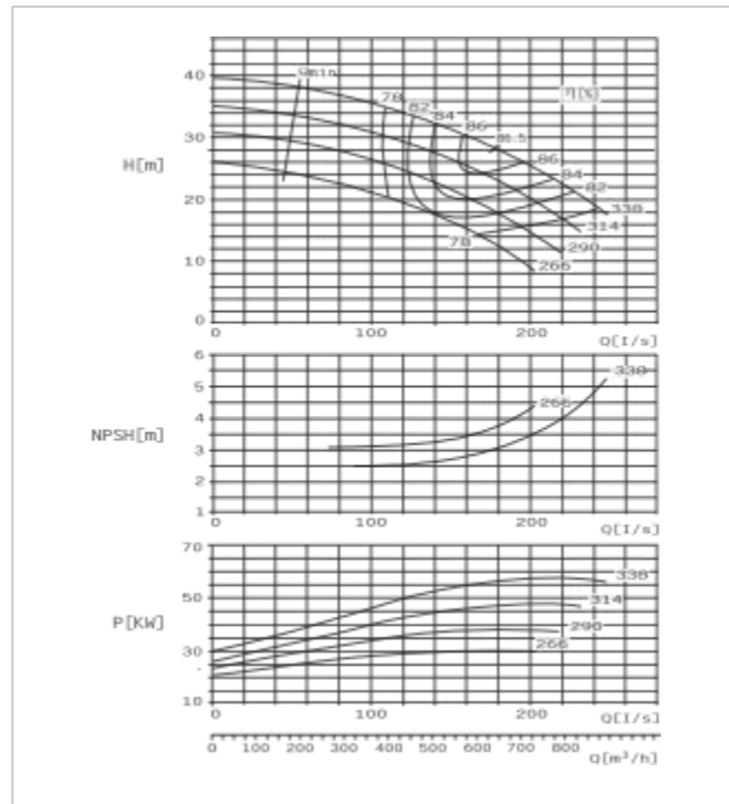
SBS200-320 F Performance Curve n=1450r/min
