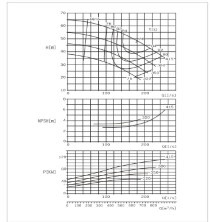
SBS200-420 F Performance Curve n=1450r/min
