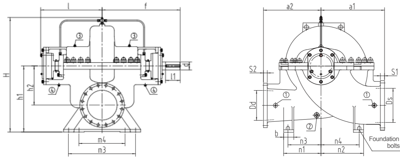
Suction flange
