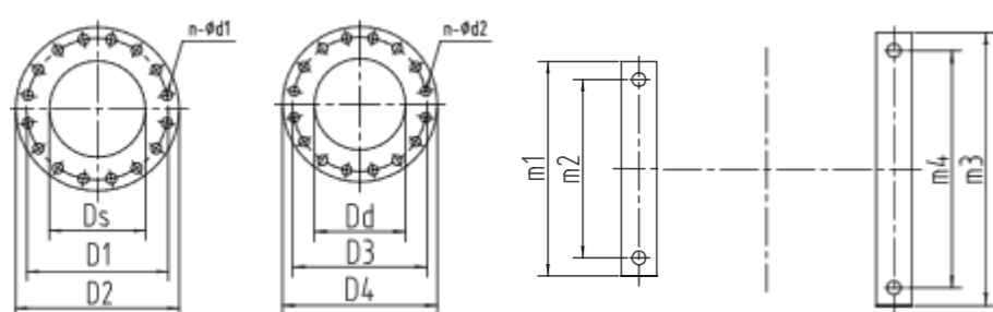
Suction flange Discharge flange
