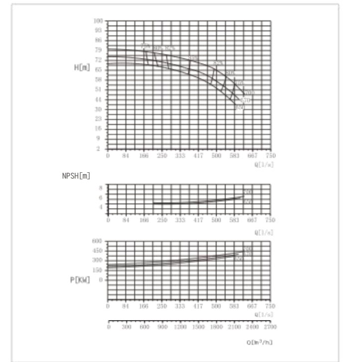
SBS350-700 Performance Curve n=960r/min
