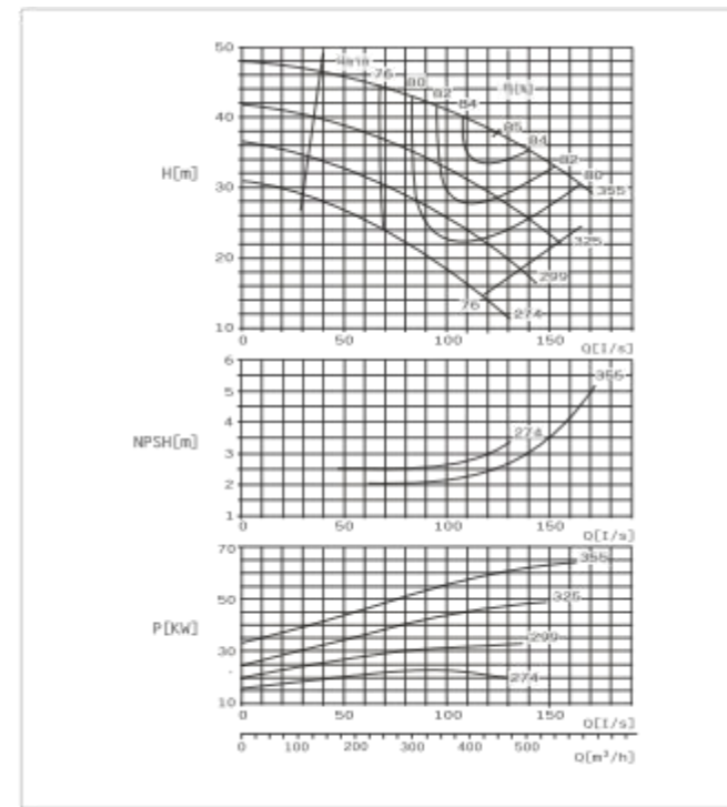
SBS150-360 E Performance Curve n=1450r/min
