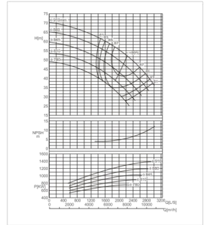
SBS800-970 F Performance Curve n=725r/min
