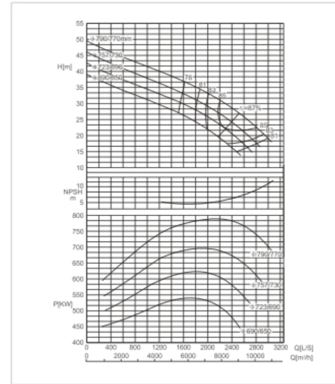
SBS800-740 E Performance Curve n=725r/min
