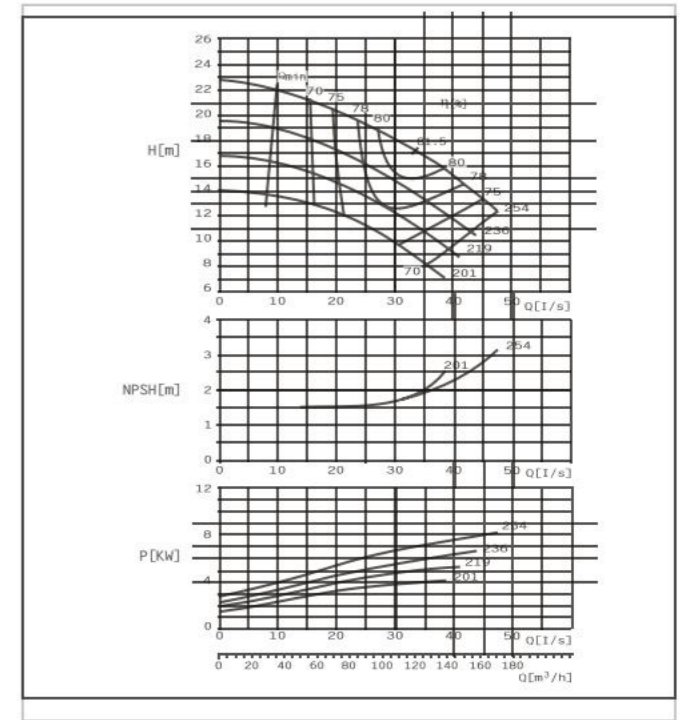
SBS100-250 F Performance Curve n=1450r/min
