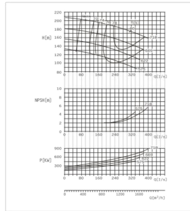
SBS250-710 E Performance Curve n=1450r/min
