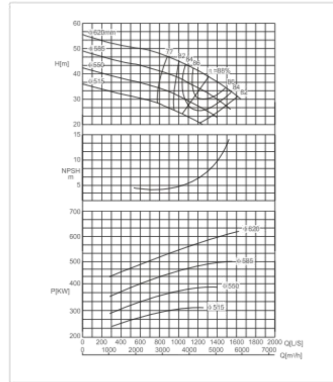
SBS600-620 E Performance Curve n=960r/min
