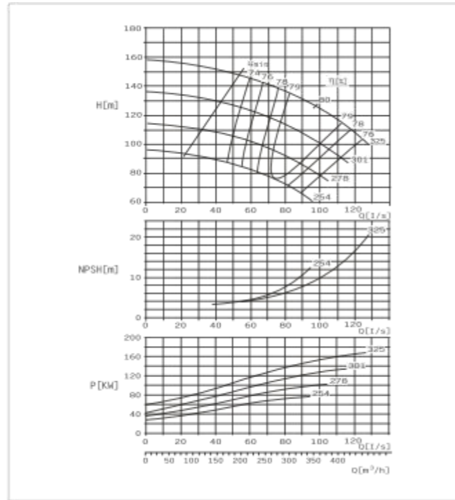
SBS100-310 EG Performance Curve n=2900r/min
