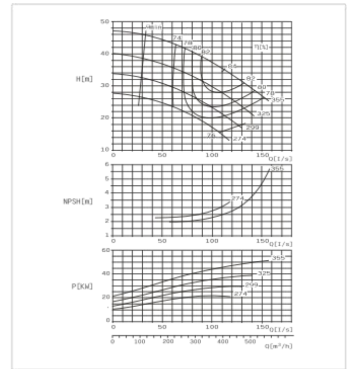
SBS150-360 F Performance Curve n=1450r/min
