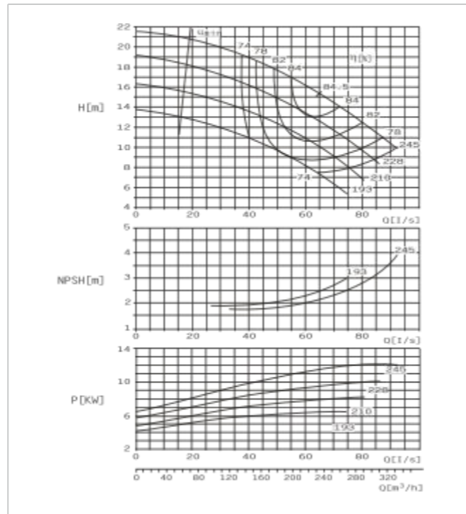
SBS125-230 F Performance Curve n=1450r/min
