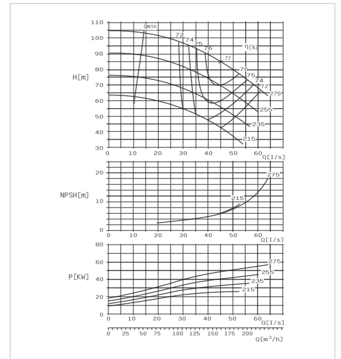
SBS80-270 FG Performance Curve n=2900r/min
