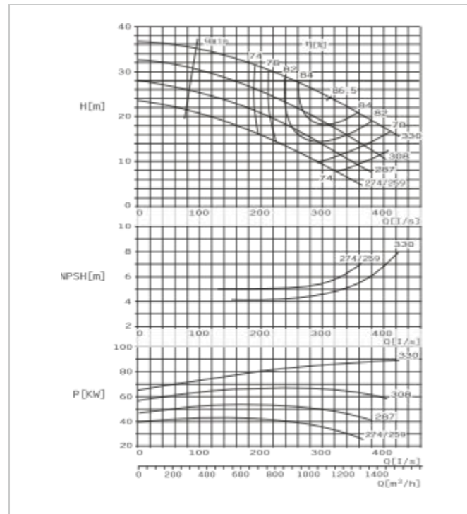
SBS300-300 E Performance Curve n=1450r/min
