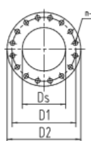
Suction flange
