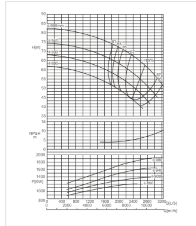
SBS800-970 E Performance Curve n=725r/min
