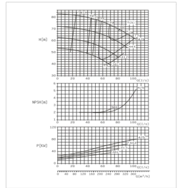
SBS125-500 F Performance Curve n=1450r/min
