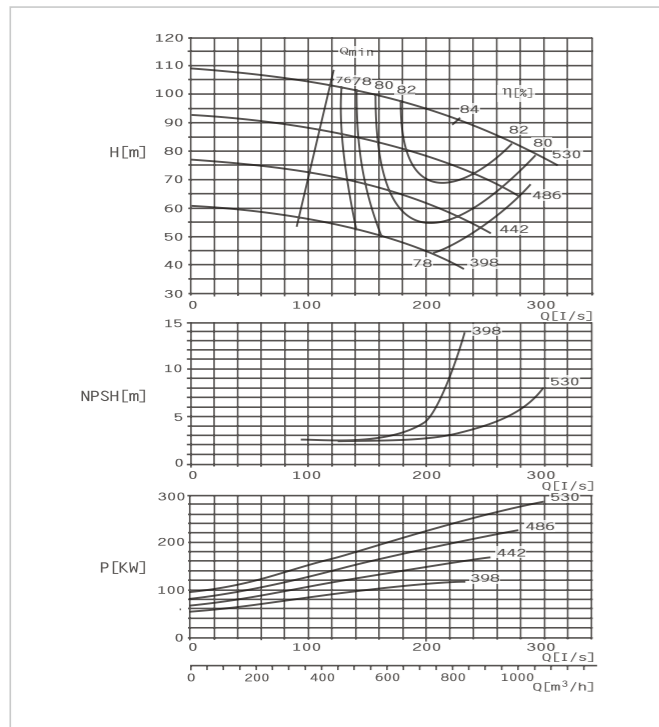
SBS200-520 E Performance Curve n=1450r/min
