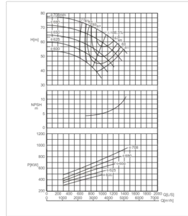
SBS500-700 E Performance Curve n=960r/min
