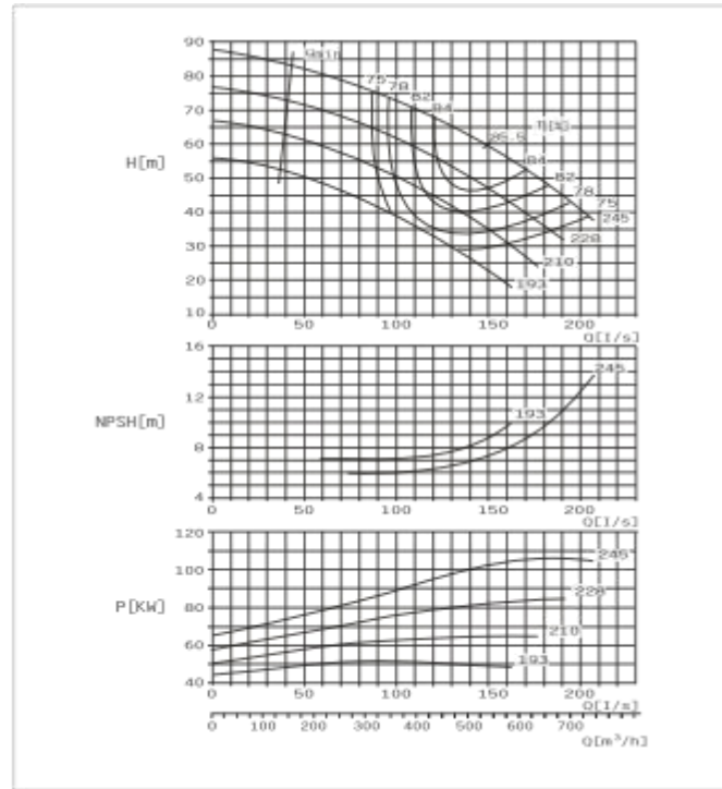
SBS125-230 EG Performance Curve n=2900r/min
