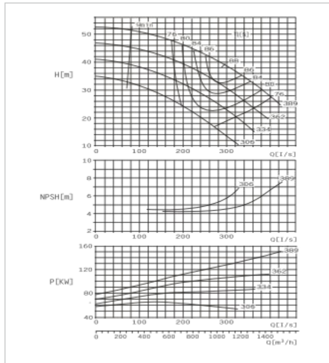
SBS250-370 E Performance Curve n=1450r/min
