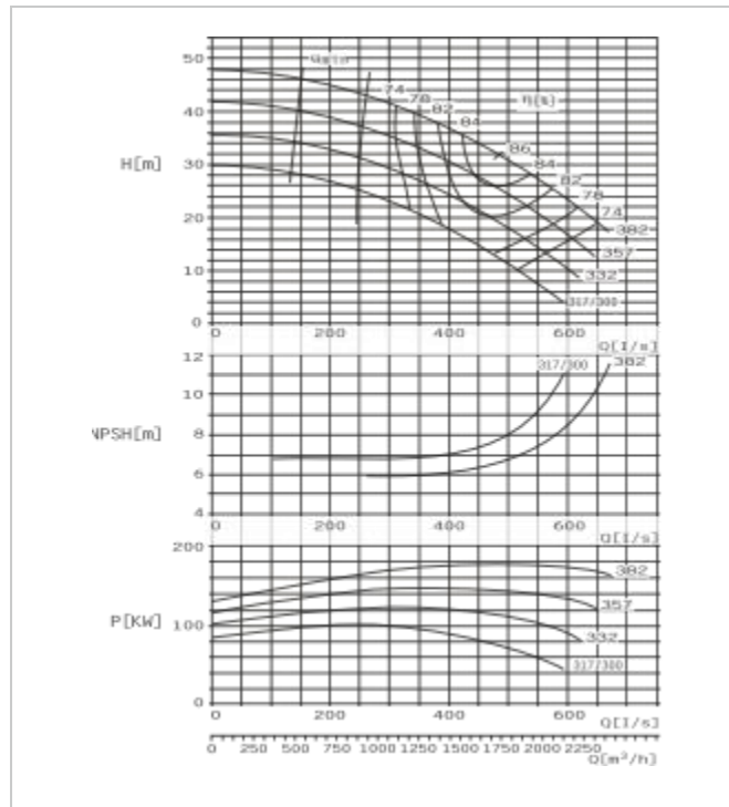
SBS350-360 E Performance Curve n=1450r/min
