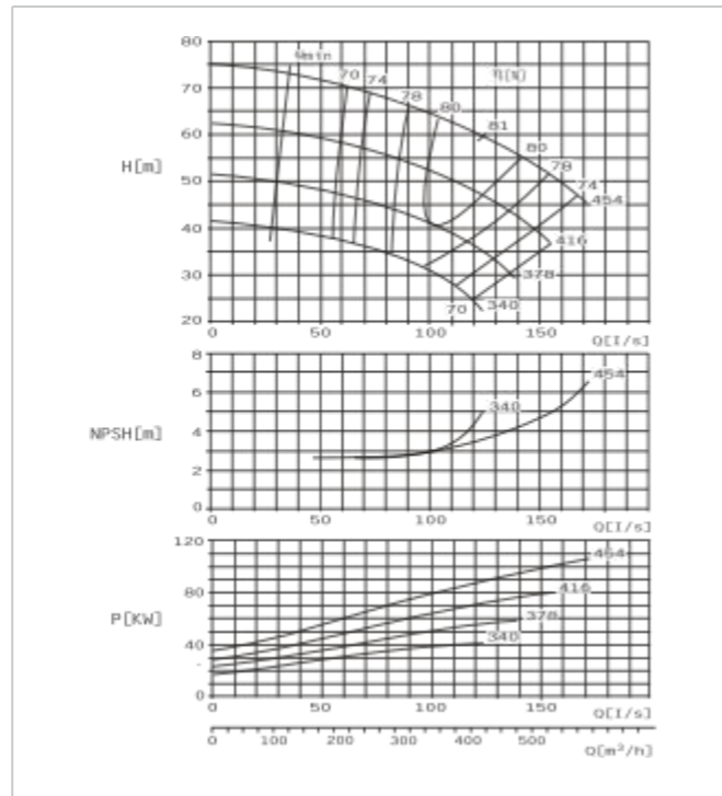
SBS150-460 F Performance Curve n=1450r/min
