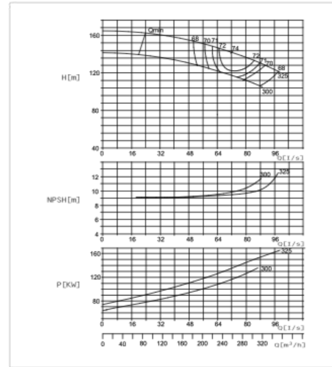
SBS100-325 EG Performance Curve n=2900r/min
